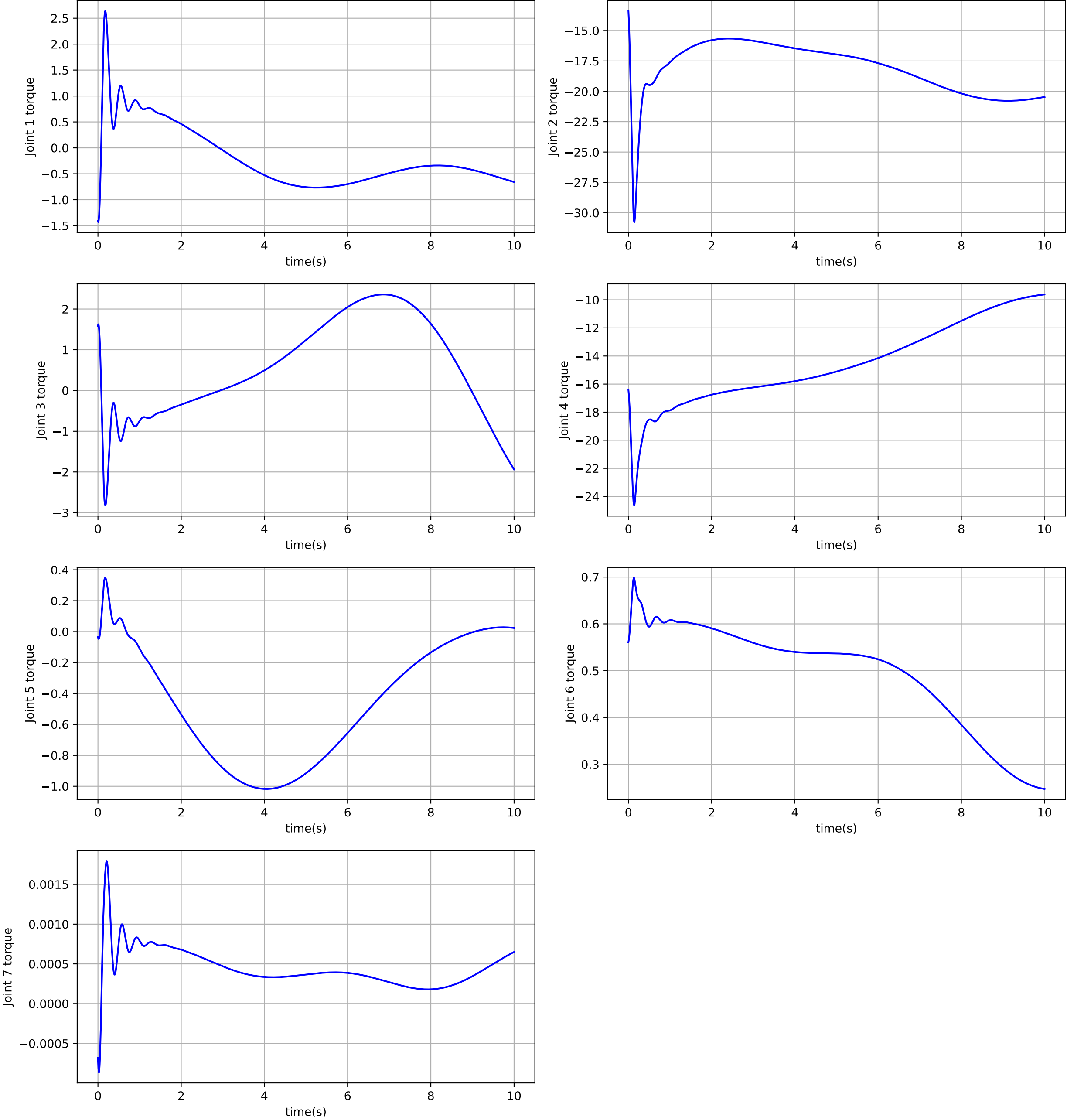
Control Inputs (S=3, S1=2, m=5)
